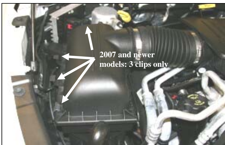
1. Disconnect the negative battery cable. Unlatch the four clips (three on 2007 and newer models) on the factory airbox.
