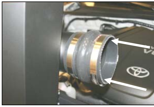
11. Install the urethane hump hose (#4), and two #72 hose clamps (#8) on the tube of the CAD as close to the panel as possible. Leave the hose clamps loose for now.
